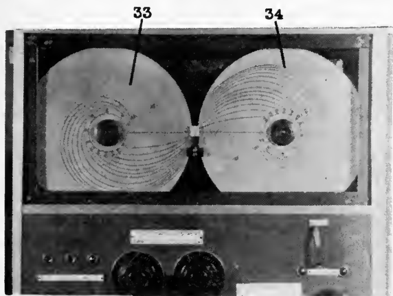
FIG. 8. Photograph of front of integrator, showing the dials. (Front panel removed.)
